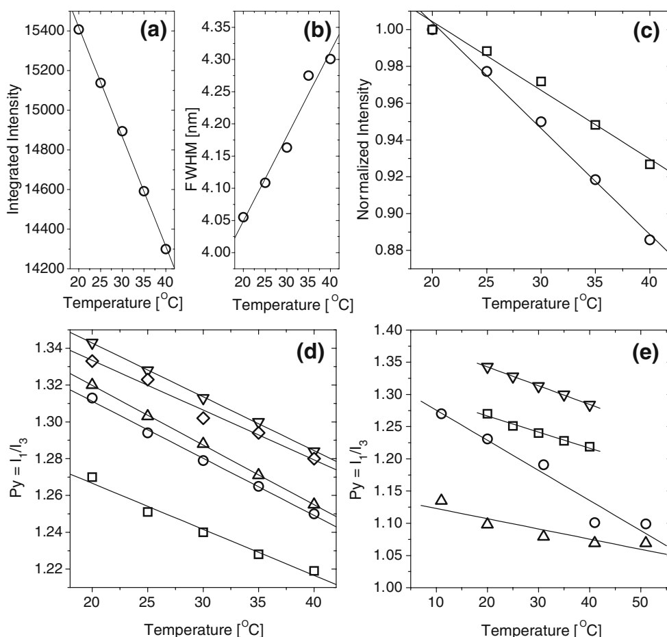
Fig. 4 Temperature dependence of: a integrated fluorescence intensity, and b the full width at half maxima (FWHM) of pyrene doped P65 copolymer film. c Temperature dependence of the intensity of the first ( I_1 ) and the third ( I_3 ) vibronic band of pyrene doped P65 copolymer film. Intensities normalized to the emission at 20°C. d Temperature dependence of the I_1/I_3 ratio ( py parameter) of pyrene doped poly(NIPAM-co-NtBA) films ( \square ) pNtBA, ( \circ ) P50, ( \Delta ) p65, ( \diamond ) p85, ( \nabla ) pNIPAM. e Comparison of the temperature dependence of the I_1/I_3 ratio as a function of temperature for ( \circ ) ethanol, ( \Delta ) 1-propanol, ( \nabla ) pNIPAM, and ( \square ) pNtBA. Data for ethanol and 1-propanol from Ref. [27]
