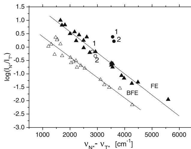
Fig. 9 Plot of the \log(I_{N^*}/I_{T^*}) ratio of dye FE ( \blacktriangle ) and BFE ( \triangle ) vs. band separation \nu_{N^*}-\nu_{T^*} in different organic solvents based on the data from Ref. [7]. Filled circles ( \bullet ) correspond to the data from FE in pNIPAM (1) and pNtBA (2). Empty circles ( \circ ) correspond to the data from BFE in pNIPAM (1) and pNtBA (2). Solid lines represents linear fits for the liquid organic solvents
