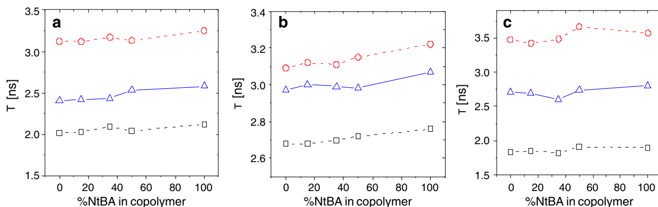
Fig. 10 Average fluorescence lifetime ( \tau ) of FE a , BFE b , and MFE c doped copolymers measured at N* band maximum ( \square ), T* band maximum ( \circ ), and all emission wavelengths ( \Delta ), using a 410 nm long pass filter
