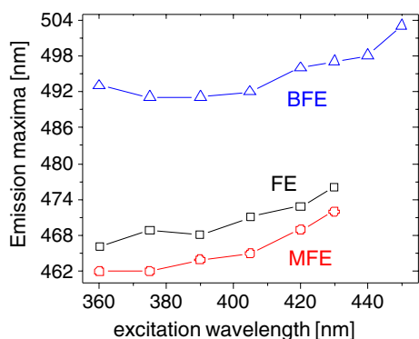
Fig. 8 Position of N^* band maxima in NIPAM-NtBA copolymer system (50% NtBA case) as a function of excitation wavelength
