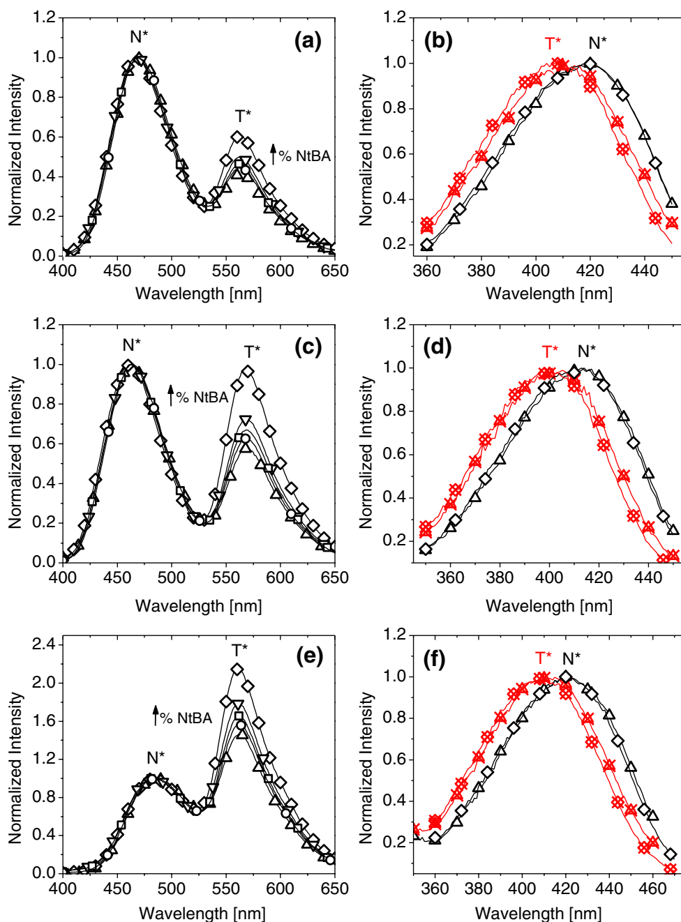
Fig. 5 Normalized fluorescence spectra (a, c, e) and excitation spectra (b, d, f) of hydroxyflavone FE (a & b), MFE (c & d), and BFE (e & f) doped copolymers. (a, c, e): NIPAM ( \Delta ), P85 ( \circ ), P65 ( \square ), P50 ( \square ), NtBA ( \diamond ), excitation wavelength 375 nm. (b, d, f): excitation spectra of NIPAM ( \Delta ), and NtBA ( \diamond ), recorded at maximum of N* ( \Delta , \diamond ) and T* , band
