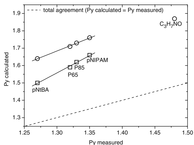
Fig. 3 Plot of measured p_y versus calculated values for poly(NIPAM-co-NtBA) films, ( \square ) p_y values obtained from Eq. 1, ( \circ ) p_y values obtained from Eq. 2
