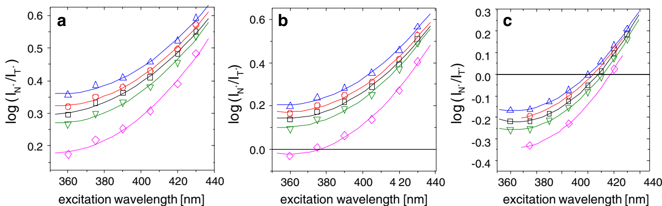
Fig. 7 Dependence of emission band ratio \log(I_{N^*}/I_{T^*}) on excitation wavelength for MFE a , FE b , and BFE c , and NIPAM ( \Delta ), P85 ( \circ ), P65 ( \square ), P50 ( \square ), NtBA ( \diamond )
