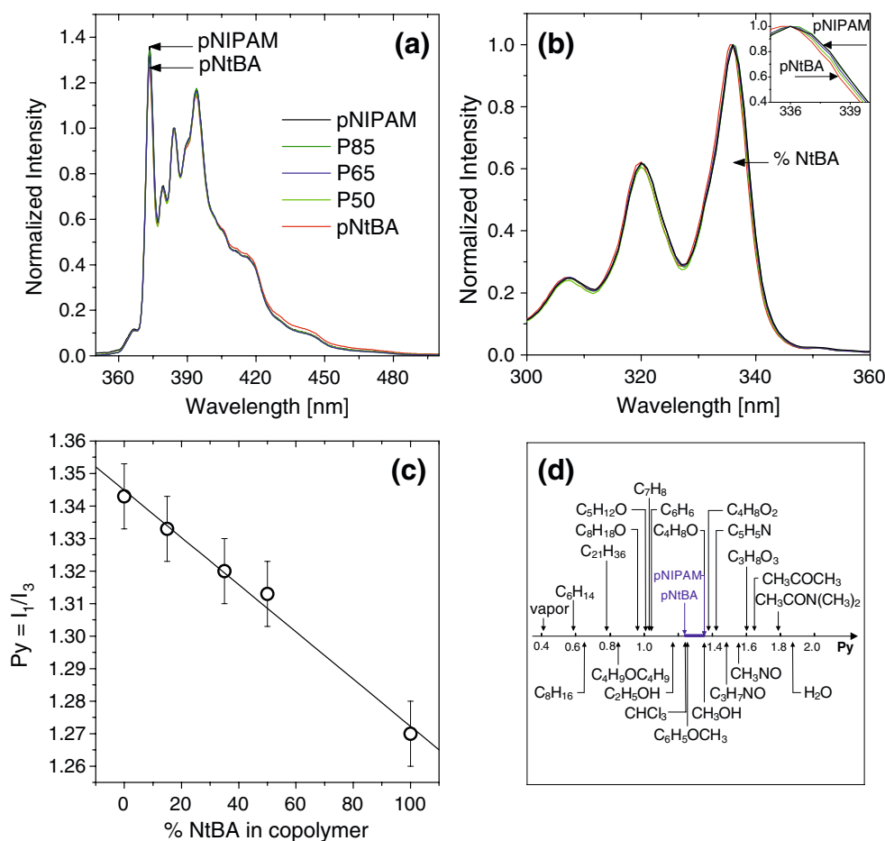
Fig. 2 a Normalized emission spectra of pyrene doped poly (NIPAM-co-NtBA) films, b normalized excitation spectra of pyrene doped poly(NIPAM-co-NtBA) films recorded at the emission of the first vibronic band, c the py values for poly (NIPAM-co-NtBA) films at 20^\circ\text{C} , and d categorization of poly(NIPAM-co-NtBA) films along the py solvent polarity scale. The py values for solvents were taken from Ref. [34]
