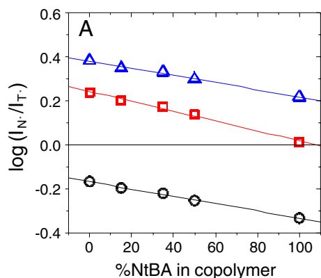
Fig. 6 Plot of \log(I_{N^*}/I_{T^*}) versus % of hydrophilic component NtBA for the hydroxyflavone MFE ( \Delta ), FE ( \square ), BFE ( \circ ) doped films, using a 375 nm excitation wavelength
