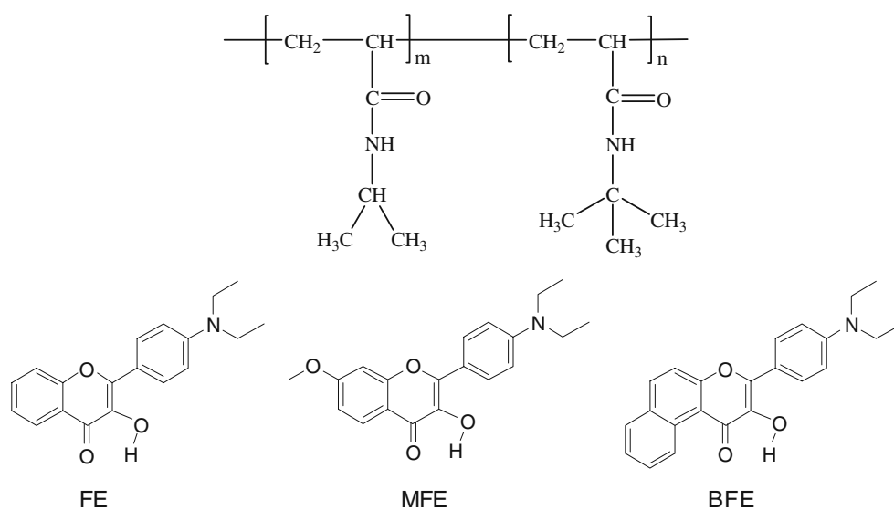
Fig. 1 Chemical structures of: a the NIPAM-co-NtBA copolymers showing the very small structural difference of one methyl group between the NIPAM and NtBA groups, b the flavone based fluorophores 4'-diethylamino-3-hydroxyflavone (FE), 5,6-benzo-4'-diethylamino-3-hydroxyflavone (BFE), and 4'-diethylamino-3-hydroxy-7-methoxyflavone (MFE) used in this study
